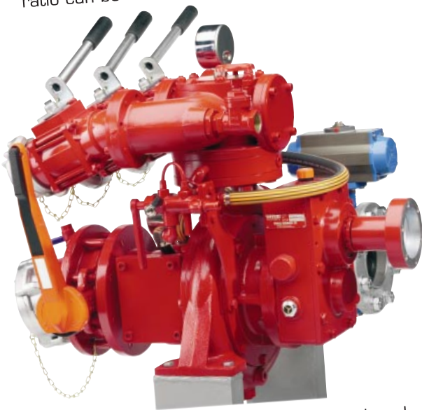
The rear mounted D-240 pump is equipped with compressed air pressure primer.
